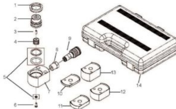
Replacement Parts Illustration for Model 5TFBK
