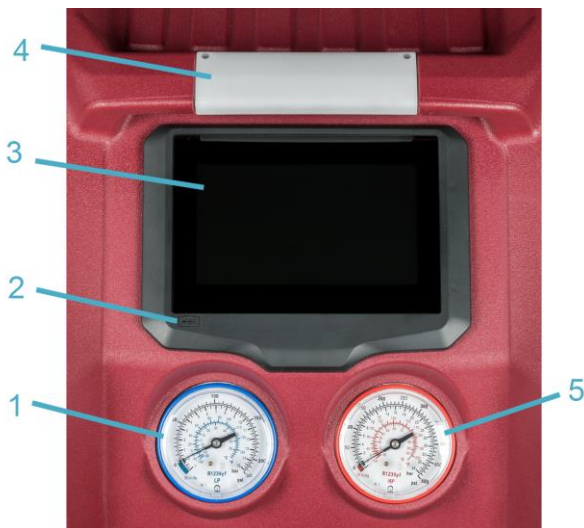
Fig. 5: Display and operating unit
