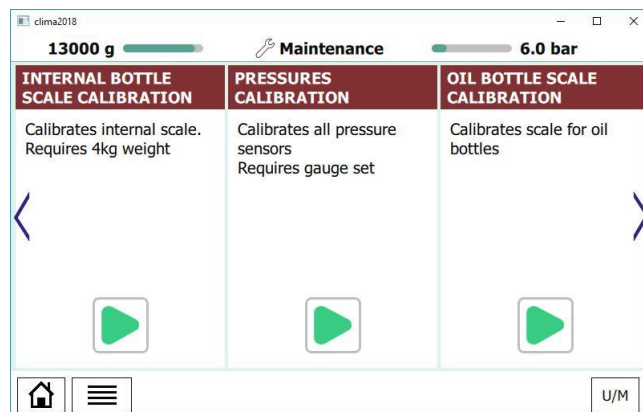
Fig. 27: Maintenance screens
