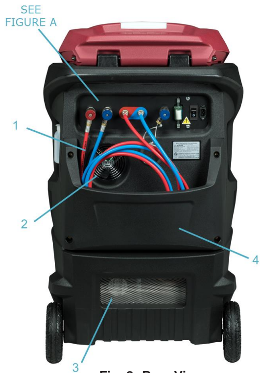
Fig. 2: Rear View
