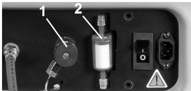
Fig. 34: Refrigerant identification unit
