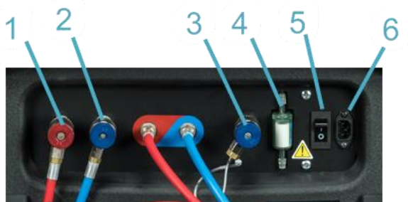
Figure A: Rear Connection View
