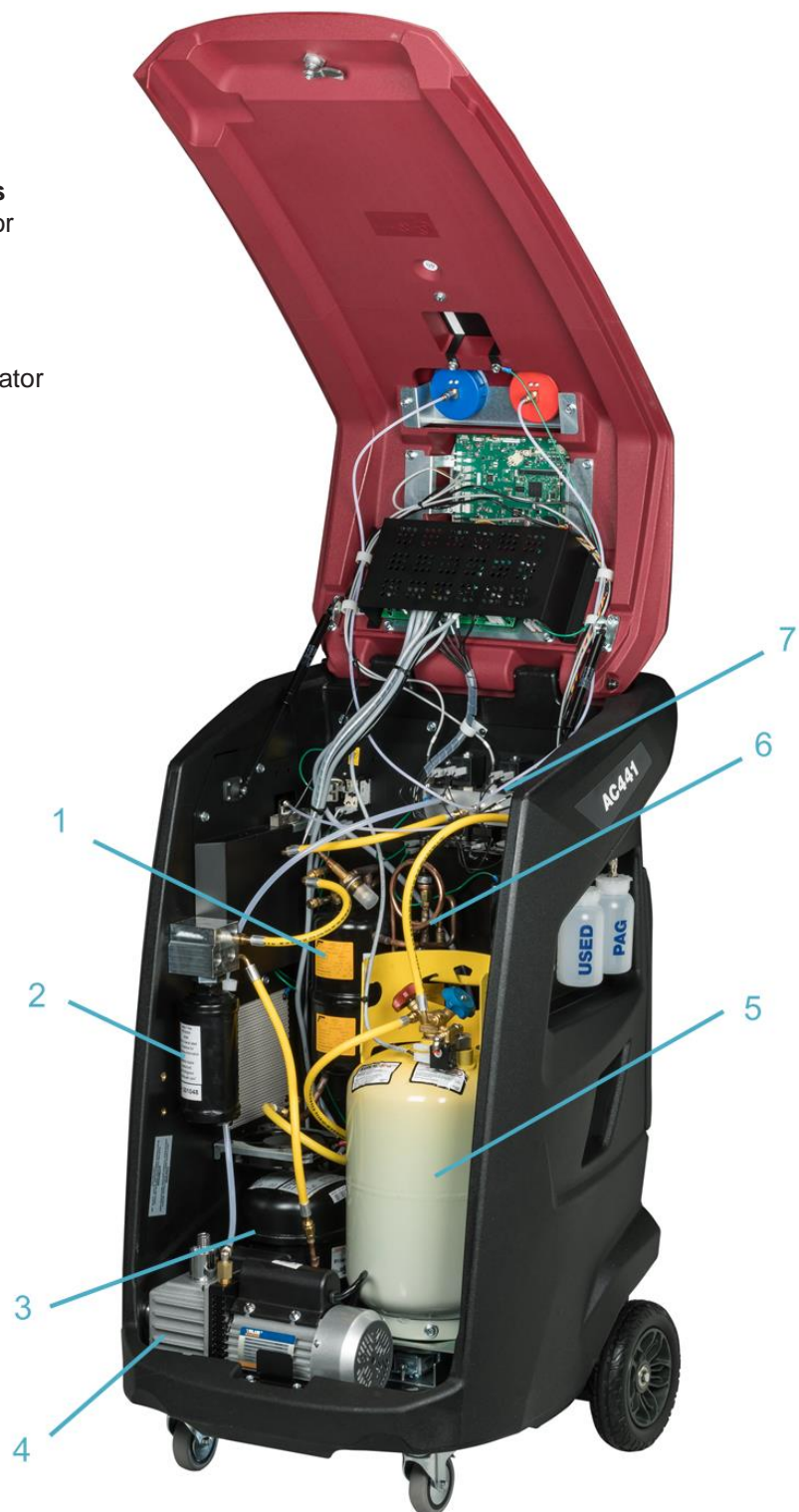
Fig. 4: Internal components
