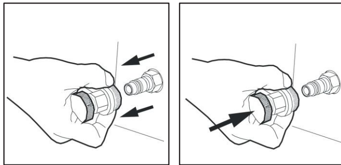
Fig. 9: Fastening quick release coupling
