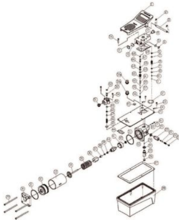
Replacement Parts Illustration for Model AFP10K
