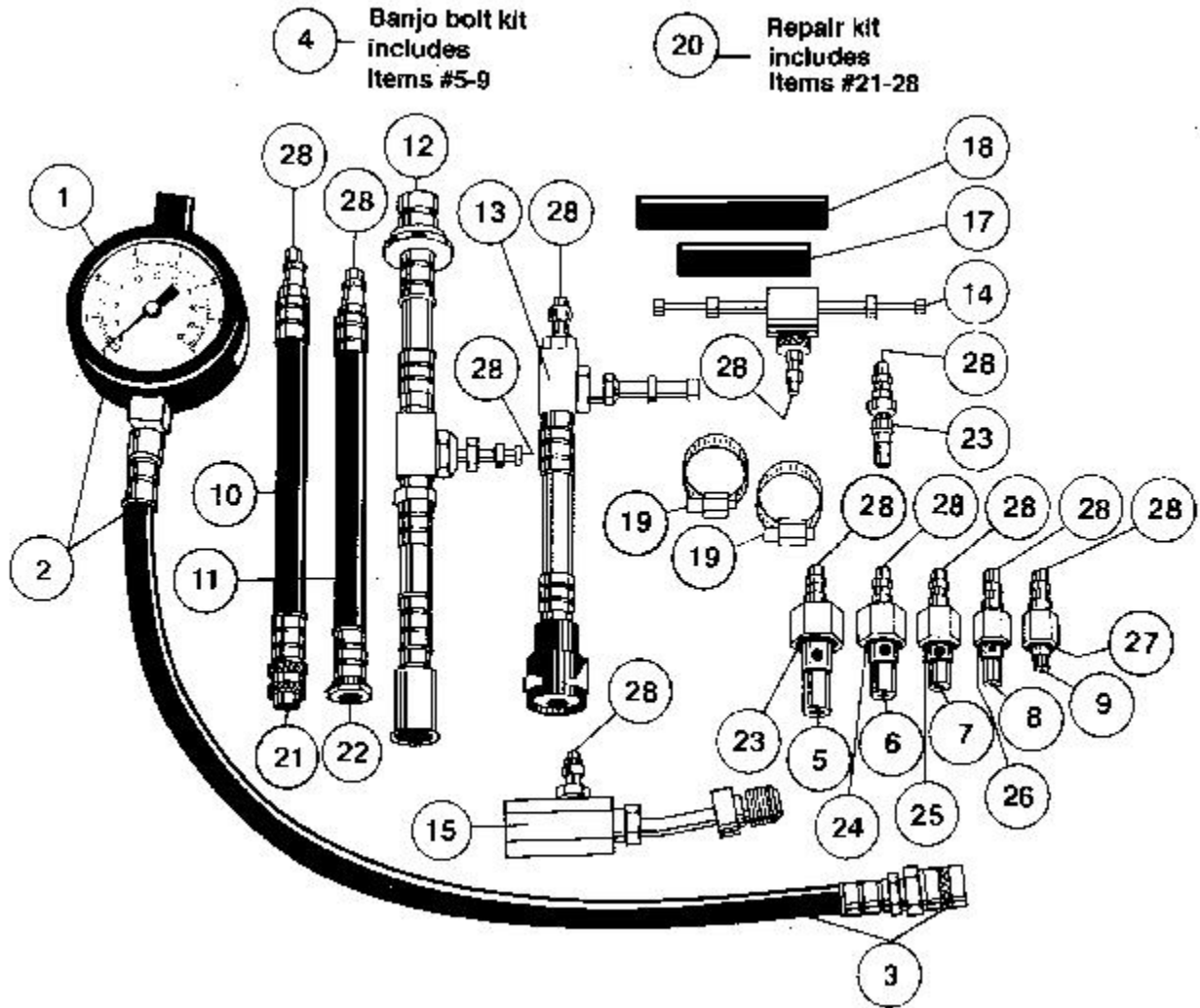
FIT448 - FUEL INJ. TESTER (NOT CIS/TBI)
