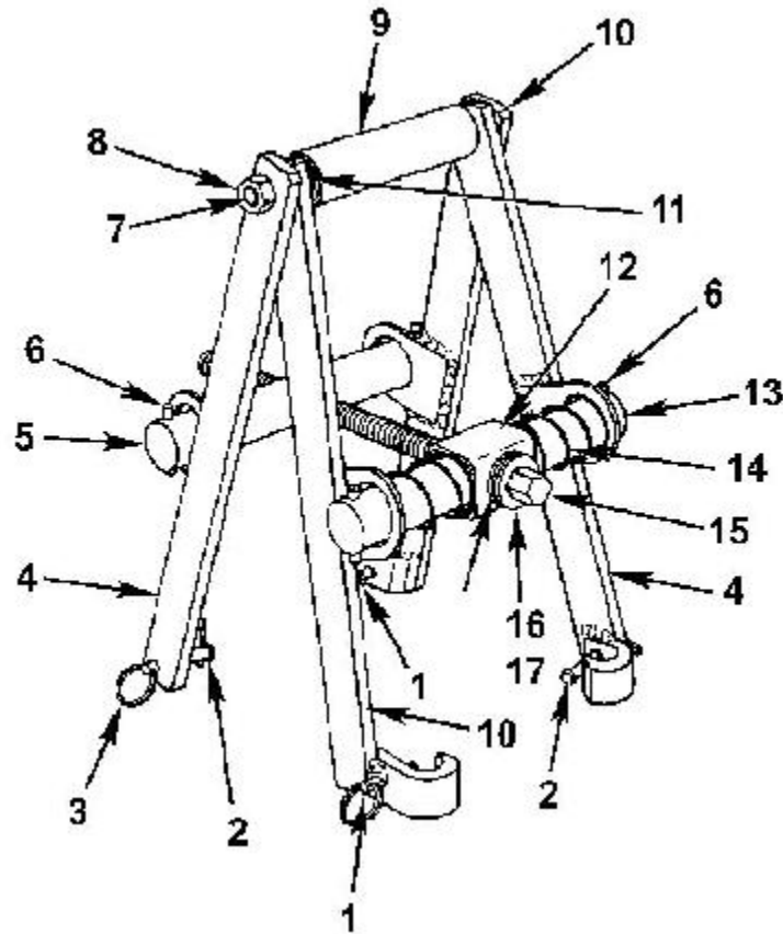
M7560 - CLAMSHELL STRUT TOOL
