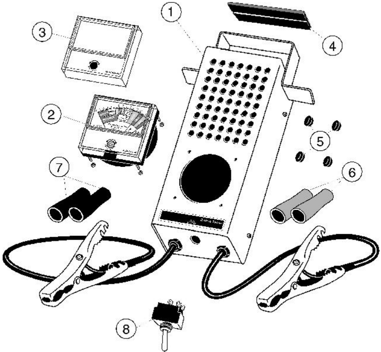
MD4260 - BATTERY LOAD TESTER
