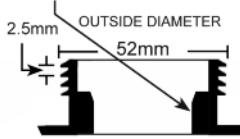
Thread Cutaway
