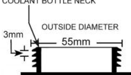
Thread Cutaway
