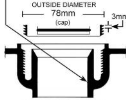
Thread Cutaway
