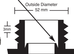
Thread Cutaway
