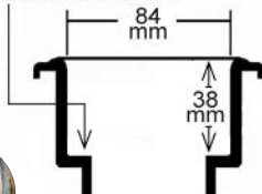
Thread Cutaway
