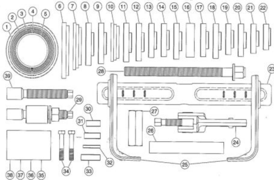
Hub Grappler Kit Carrying Case Layout
