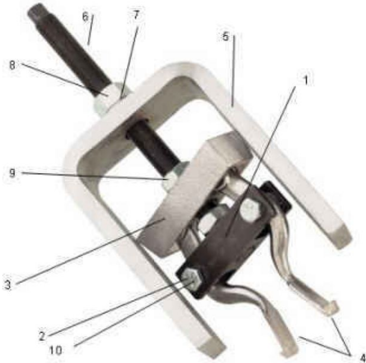
MST7318 - PILOT BEARING PULLER
