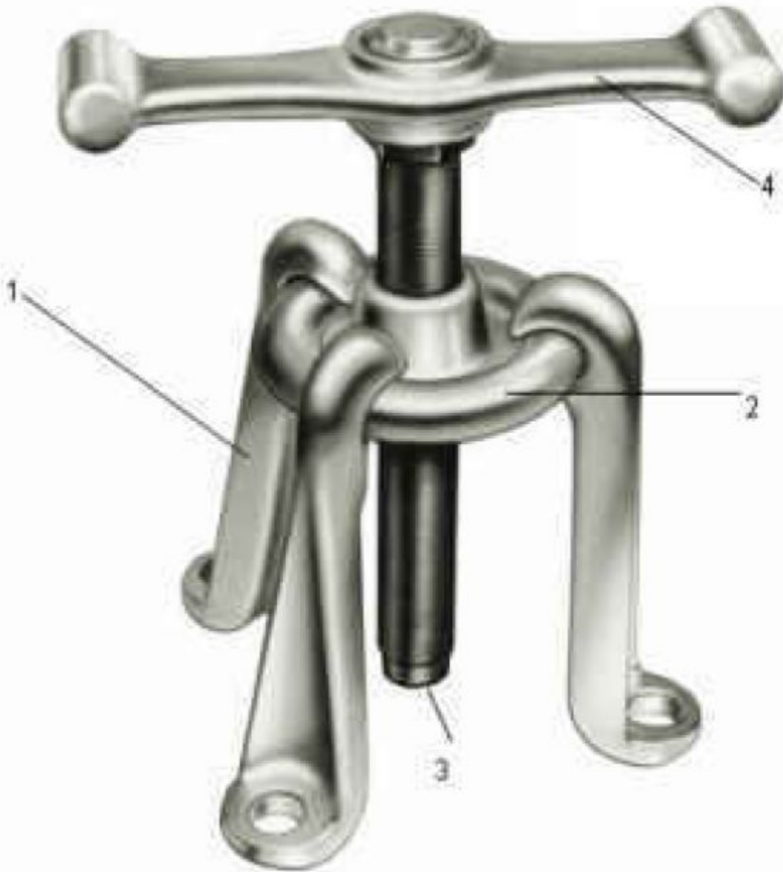
MST7394 - UNIVERSAL HUB PULLER
